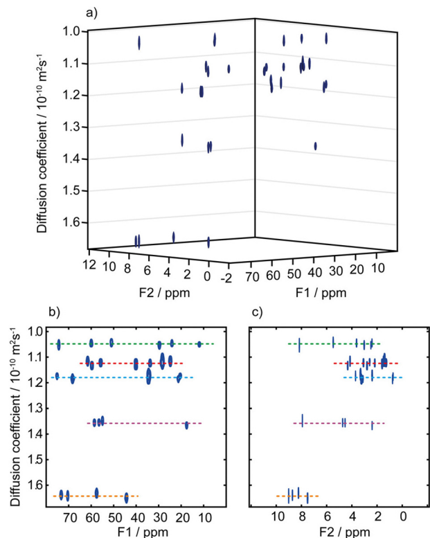
Fig. 3 (a) Pseudo-3D DOSY plot of the Oneshot-HSQC spectrum of mixture of five B vitamins (biotin, B7; pyridoxine hydrochloride, B6; pantothenic acid calcium complex, B5; niacin, B3; and thiamine hydrochloride, B1) in DMSO- d_6 . (b) 2D projection along F_2 , and (c) 2D projection along F_1 . F_1 and F_2 are the ^{13}\text{C} and ^1\text{H} dimensions, respectively. Dashed lines are used to aid visualization and indicate the peaks of biotin, B7 (red); pyridoxine hydrochloride, B6 (purple); pantothenic acid, B5 (blue); niacin, B3 (orange); and thiamine hydrochloride, B1 (green). The spectra from the five components are easily distinguished, with diffusion coefficients of (1.05, 1.12, 1.18, 1.36, \text{ and } 1.64) \times 10^{-10} \text{ m}^2 \text{ s}^{-1} for vitamins B1, B7, B5, B6, and B3, respectively. Data acquisition took 45 h, but a much shorter acquisition would have sufficed. Reproduced with permission from ref. 51, © 2018 American Chemical Society.
