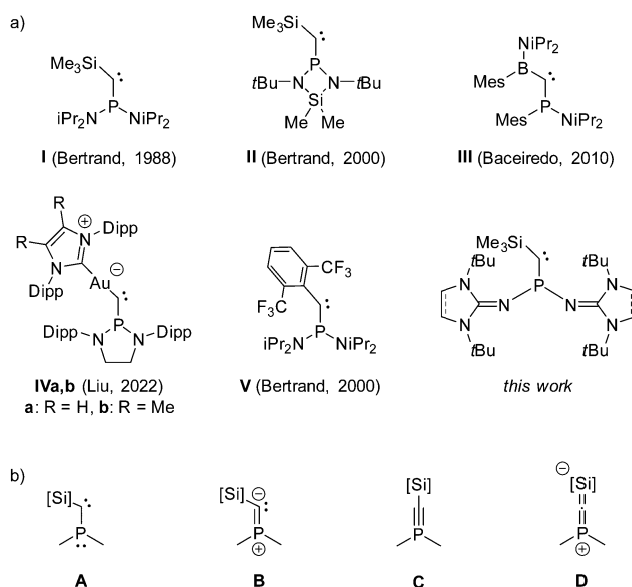
Fig. 1 (a) Selected examples of phosphino(silyl)carbenes and the phosphino(silyl)carbene presented in this work. Dipp = 2,6-diisopropylphenyl. (b) Possible electronic structures of phosphino(silyl)carbenes ([Si] = silyl group).
