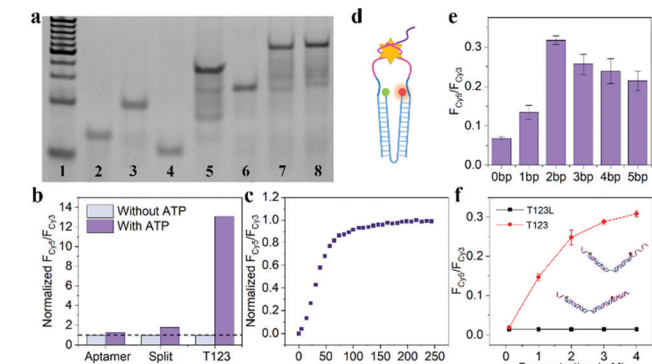
Fig. 2 (a) Gel electrophoresis. Line 1–8: 20 bp marker, T1, T2, T3, T1 + T2, T1 + T3, T1 + T2 + T3, T1 + T2 + T3 + Lock. (b) The response of ATP aptamer, split aptamer and T123 to ATP. The background signals were normalized separately (dotted line). (c) Time-dependent fluorescence spectra of T123 in response to 2 mM ATP. (d) Schematic diagram of the nano-tweezers. (e) The probe with a different number of inserted bases were utilized as a target model. (f) Fluorescence spectra of the T123 and T123L responding to ATP at different concentrations, respectively. The samples were excited at 525 nm.
