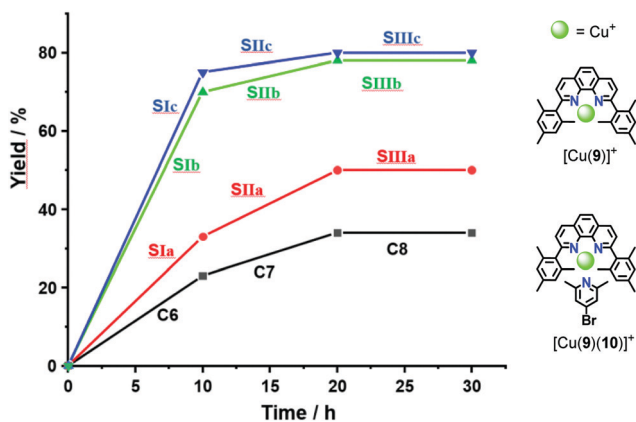
Fig. 4 Yield of the click product 8 (from 6 and 7 , each c = 1.20 \times 10^{-2} M) in states SIIa-c , SIIa-c (each c = 40.0 \times 10^{-6} M) and with model complexes C6 = [Cu(9)] + , C7 = [Cu(9)(10)] + ( c = 1.20 \times 10^{-3} M) after 10 h at 40 °C for each state.
