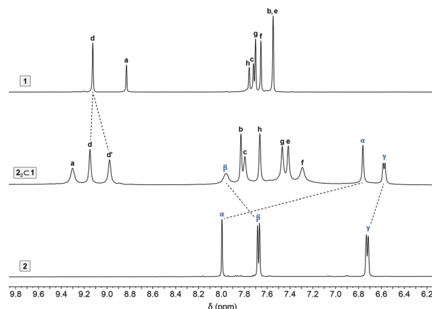
Fig. 2 Partial 1 H NMR spectra of cage 1 (top), indigo carmine 2 (bottom), and 2_2 \subset 1 (middle) (500 MHz, \text{D}_2\text{O} , 298 K). For the full-range spectrum of 2_2 \subset 1 , see Fig. S2 in the ESI†.
