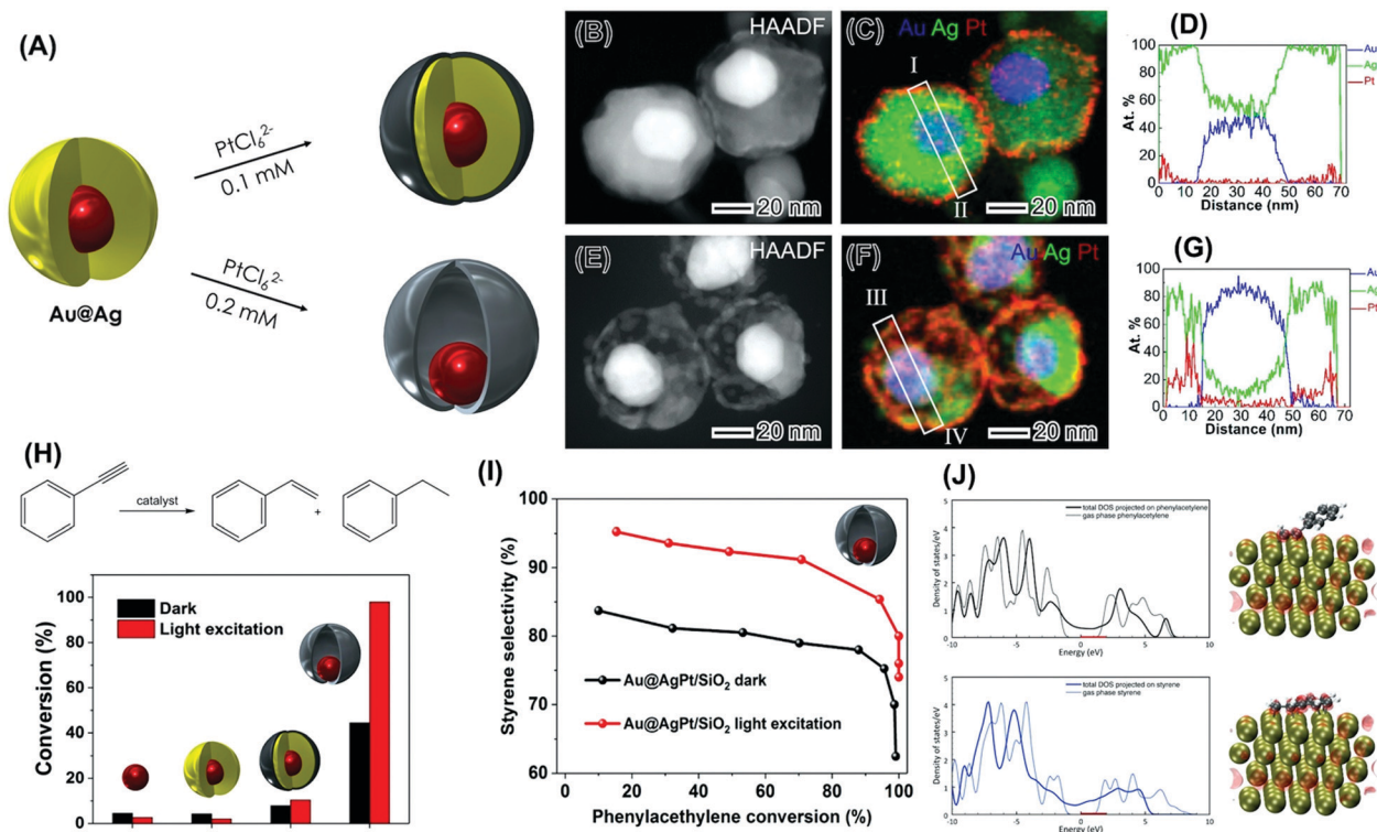
Fig. 9 (A) Synthesis of plasmonic-catalytic Au@Ag@Pt core-shell (top) and Au@AgPt nanorattles (bottom) via the galvanic replacement reaction between PtCl 6 2- (aq) and Ag in Au@Ag core-shell NPs. 100 (B–G) STEM analysis for Au@Ag@Pt core-shell (B–D) and Au@AgPt nanorattles (E–G). 100 (B and E) HAADF image in which the brightest contrast from Au core results from its higher Z (atomic number) as Z_{\text{Au}} > Z_{\text{Pt}} > Z_{\text{Ag}} ; (C and F) Corresponding composite elemental map EDS elemental maps of Au (blue), Ag (green), and Pt (red). (D and G) Atomic-percent distribution from quantified EDS line scan along the line I–II (D) marked in (C) and along line III–IV (G) marked in (F). (H) Scheme for the phenylacetylene hydrogenation reaction leading to the formation of styrene and ethylbenzene and conversion (%) in the dark and under visible light excitation (black and red bars, respectively) employing supported Au, Au@Ag, Au@Ag@Pt core-shell NPs, and Au@AgPt nanorattles as catalysts. (I) Styrene selectivity as a function of conversion percentages for Au@AgPt nanorattles under dark (black trace) and visible light excitation conditions (red trace). 100 (J) DFT-calculated projected density of states of phenylacetylene (top panel) and styrene (bottom panel) in the gas phase (dotted trace) and adsorbed on Pt (solid trace). The optimized structure and integrated state from the Fermi Level (0 eV) to 2 eV are also shown. 100 Reprinted (adapted) with permission from ref. 100. Copyright 2018 American Chemical Society.
