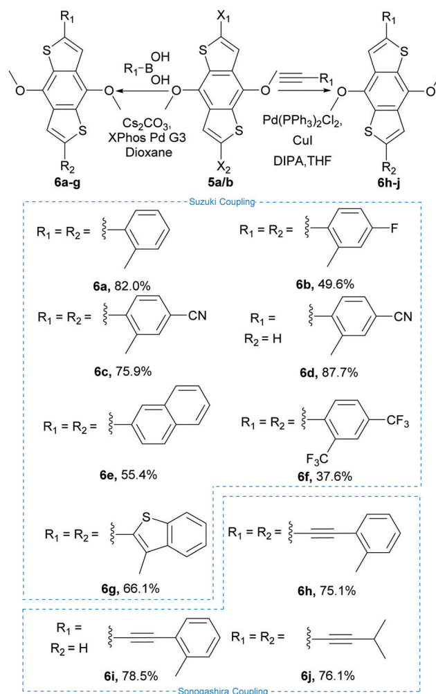
Scheme 2 Suzuki and Sonogashira reactions and yields utilized to produce species 6a–j .
