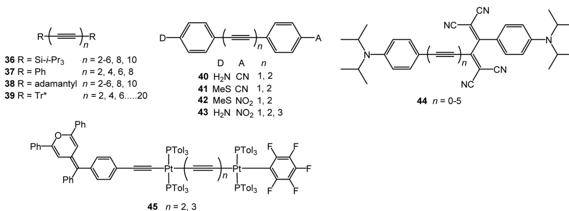
Fig. 15 Structures of 36–45 .
