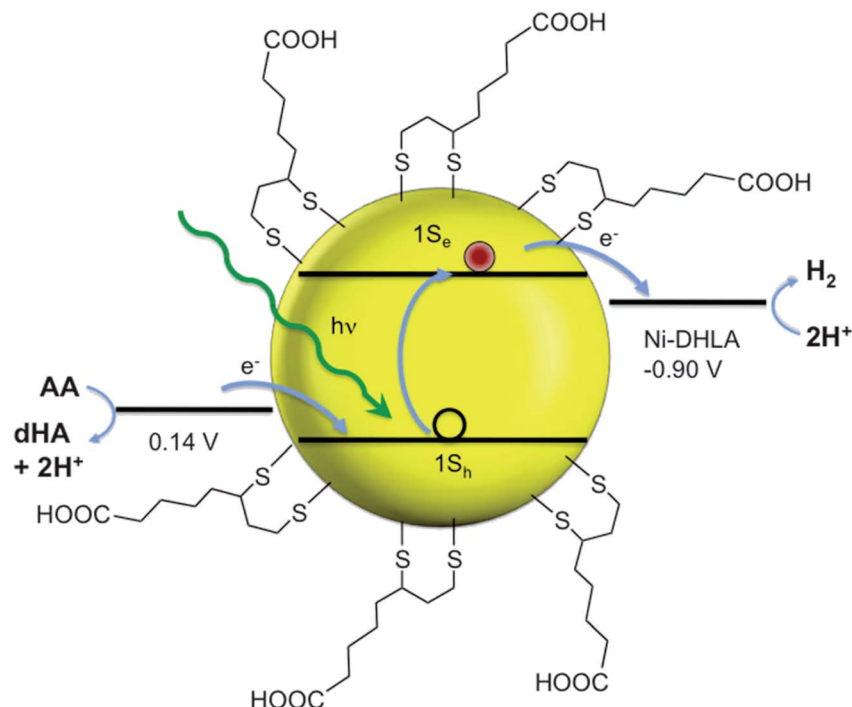
Scheme 12 Schematic diagram of the photocatalytic H 2 production by Ni 2+ -DHLA-CdSe QDs. Reproduced with permission from ref. 80, Copyright 2012, American Association for the Advancement of Science.
