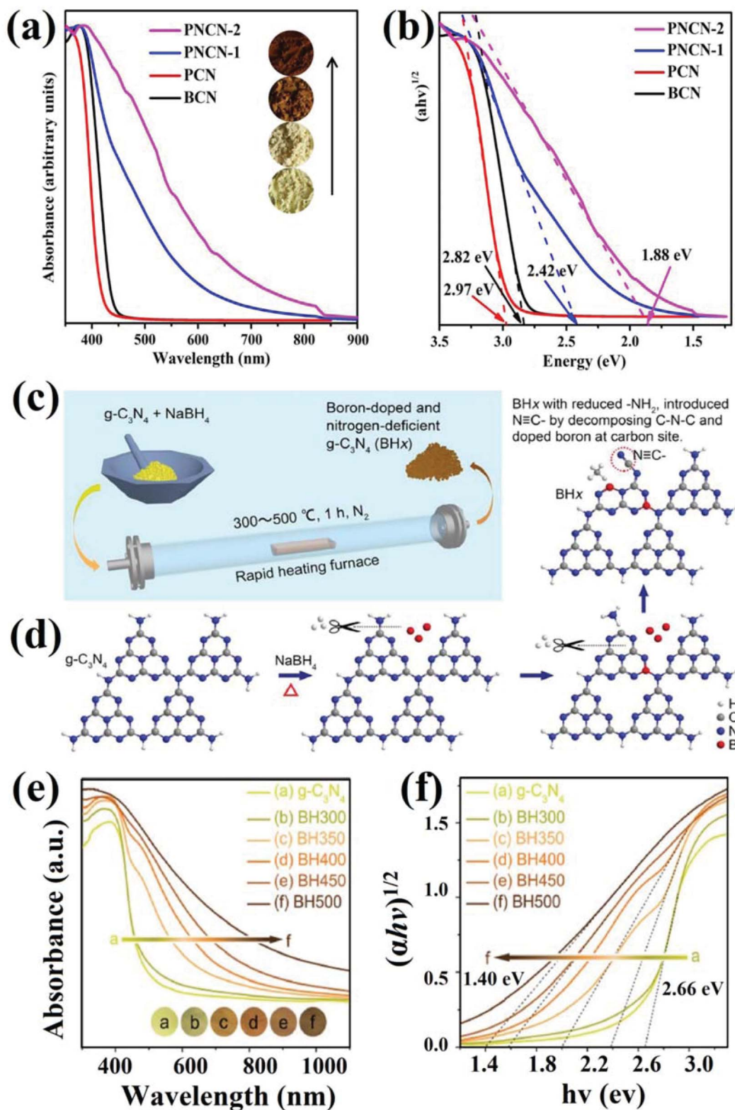
Fig. 12 Schematic illustration of (a) UV-vis DRS spectra and (b) plots representing (ah\nu)^{1/2} vs. photon energy (adapted with permission under license no. 4792401424595, Copyright 2020 Elsevier). 93 (c) Diagrammatic representation of the synthesis mechanism of defective BHx sample and (d) possible changes in the structural framework of GCN by thermal treatment. Schematic representation of (e) UV-vis DRS plots of various defect induced BHx samples prepared under different temperatures and (f) plots depicting the transformed Kubelka–Munk function vs. energy (adapted with permission under license no. 4792910600654, Copyright 2019 Wiley). 94
