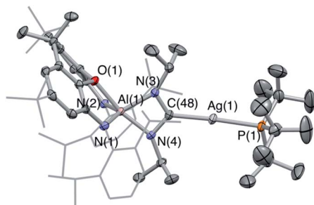
Fig. 4 Molecular structure of 5-Ag in the solid state as determined by X-ray crystallography. Thermal ellipsoids set at the 50% probability level. Hydrogen atoms omitted and ^1\text{Pr}/^1\text{Bu} shown in wireframe for clarity. Key bond lengths (Å) and angles ( ^\circ ): \text{Ag}(1)\text{--C}(48) : 2.118(2), \text{Ag}(1)\text{--P}(1) : 2.3851(6), \text{N}(3)\text{--C}(48) : 1.346(3), \text{N}(4)\text{--C}(48) : 1.345(3).
