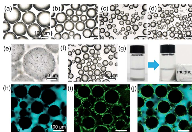
Fig. 3 Optical microscope images of Pickering emulsions stabilized by ML-HPMs at different concentrations, respectively: (a) 0.25%, (b) 0.5%, (c) 1%, and (d) 2%; the ratio of toluene to water was 3 : 1. All scale bars are 100 μm; (e)–(j) further characterization of (c): optical microscope images of the (e) interfacial structure of droplets and the (f) emulsion after one month storage, (g) exhibition of magnetic responsiveness, and (h)–(j) CLSM images; ML-HPMs and toluene were stained with FITC (green) and pyrene (cyan), respectively; all scale bars are 100 μm.
