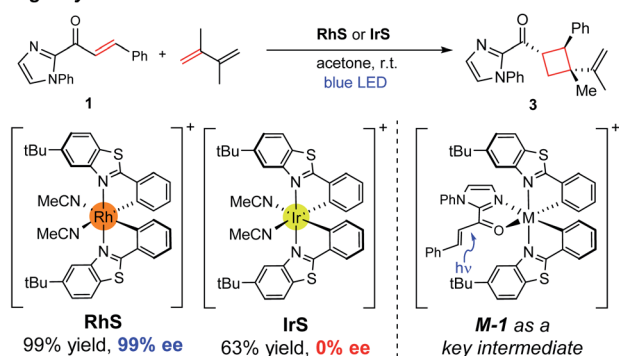
Scheme 1 Experimental conditions of the enantioselective [2 + 2] cycloaddition reaction investigated in this study.
