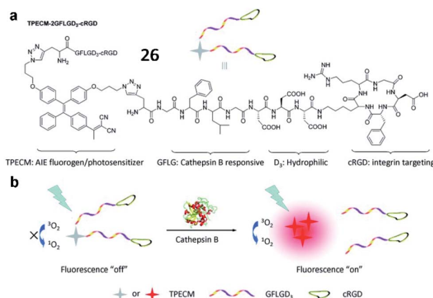
Fig. 22 The chemical structure of probe 26 and the proposed chemical conversion in response to cathepsin B. Reprinted from ref. 82 with permission. Copyright 2016 American Chemical Society.
