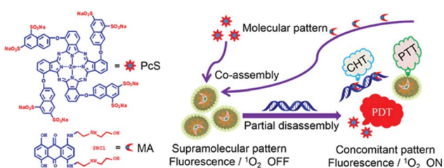
Fig. 10 Structures of octasulfonated phthalocyanine (PcS) and mitoxantrone (MA) and schematic illustration of the construction of the PcS-MA nanotheranostic agent. Adapted with permission from ref. 107. Copyright 2018, American Chemical Society.
