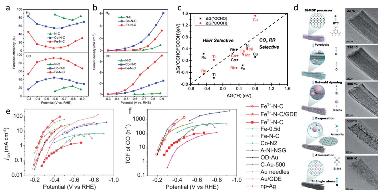
Fig. 2 The Faradaic efficiencies for CO and \text{H}_2 (a) and the current densities (b) of N–C, Co–N–C, and Fe–N–C. Reproduced from ref. 58 with permission from the American Chemical Society, copyright 2018. (c) Gibbs free energy changes for the first protonation step. Reproduced from ref. 63 with permission from The Royal Society of Chemistry, copyright 2018. (d) A schematic illustration of the process of Bi-MOF transformation to single Bi atoms and TEM images of Bi-MOF pyrolyzed at different temperatures. Reproduced from ref. 64 with permission from the American Chemical Society, copyright 2019. (e) CO current density ( j_{\text{CO}} ) and (f) apparent TOFs of CO production of \text{Fe}^{3+} –N–C and of \text{Fe}^{2+} –N–C in comparison with other reported catalysts. Reproduced from ref. 59 with permission from the American Association for the Advancement of Science, copyright 2019.
