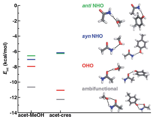
Fig. 2 Comparison of interaction energies ( E_{int} ) in kcal mol -1 of HB conformations in acetamide–methanol (acet-MeOH, left lines) and acetamide– p -cresol (acet-cres, right lines) models. The four conformations compared are the anti N–H \cdots O ( anti NHO, in green), syn N–H \cdots O ( syn NHO, in blue), O–H \cdots O (OHO, in red), and ambifunctional HBs (ambifunctional, in gray), and optimized model structures (carbon in gray, hydrogen in white, oxygen in red, and nitrogen in blue) are shown with hydrogen bonds drawn as black dotted lines.
