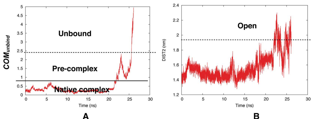
Fig. 22 Time evolution of COM_{unbind} during metadynamics simulations (A). Plotting DIST_2 as a function of time shows how flap opening is necessary in order to transit from pre-complex to unbound state. The conserved Tyr remained in gauche + conformation during the unbinding process. The simulation was carried out using PlmII-ligand complex (PDB ID:4Y6M 76 ).
