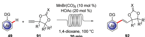
(a) Manganese(I)-catalyzed hydroarylations in flow
