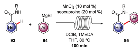
(b) Manganese(II)-catalyzed C–H arylations in flow
