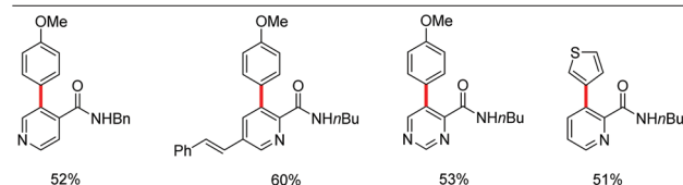
Scheme 33 Manganese-catalyzed C–H activation in flow.
