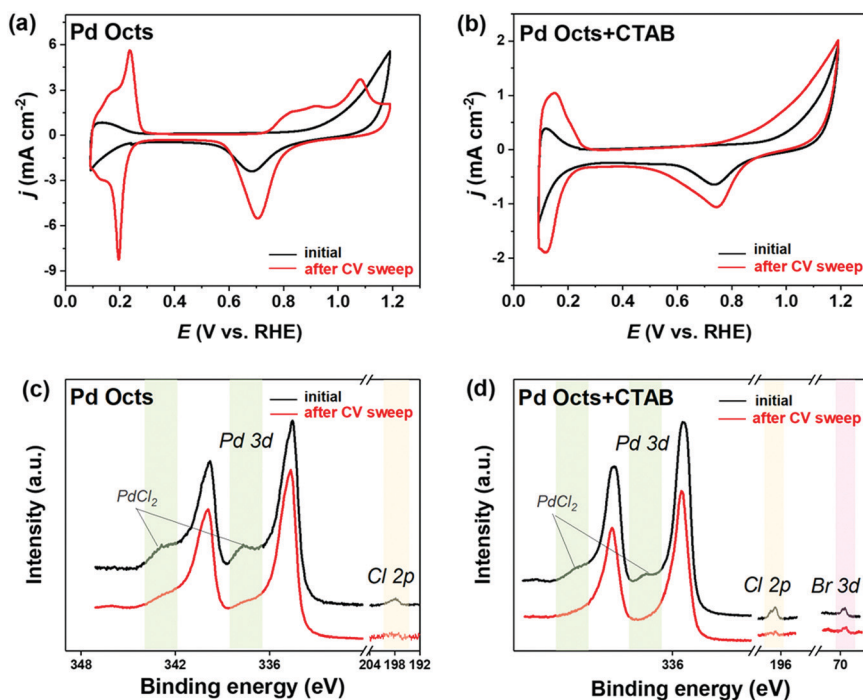
Fig. 4 Comparison of electrochemical surface cleaning for Pd Octs and Pd Octs with CTAB in 0.5 M H _2 SO _4 . (a and b) CVs and (c and d) XPS profiles of (a and c) Pd Octs and (b and d) Pd Octs with CTAB, before and after surface cleaning by CV sweeping.
