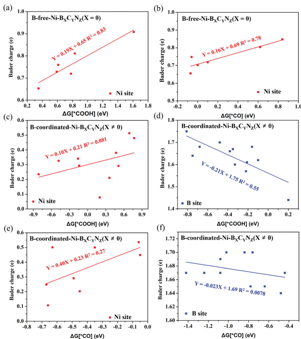
Fig. 6 Bader charge analysis of active sites (Ni or B atom) on *COOH and *CO adsorbed Ni-B X C Y N Z . Correlations of the adsorption free energy of *COOH (a) and *CO (b) intermediates with Ni Bader charge on B-free Ni-B X C Y N Z (X = 0). Correlations of the adsorption free energy of *COOH and *CO intermediates with Ni (c, e) and B Bader charge (d, f) on B-coordinated Ni-B X C Y N Z (X ≠ 0).
