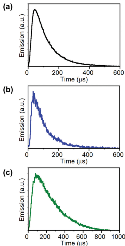
Fig. 4 Kinetic profiles of the emission in channel 2 (C2: 515–580 nm) of (a) UC Er,2 , (b) UC Ho , and in channel 1 (C1: 420–500 nm) of (c) UC Tm . ( \lambda_{\text{exc}} = 975 \text{ nm} ; F_d = 0.2 \text{ J cm}^{-2} ).
