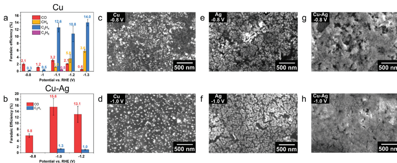
Fig. 6 (a and b) Faradaic efficiency of drop-casted Cu (a) and \text{Cu}_{1.0}\text{-Ag}_{1.0} (b) NP electrodes for CO 2 RR at various potentials for 1 h in CO 2 saturated 0.1 M KHCO 3 . (c and d) SEM images of drop-casted Cu NP films after CO 2 RR at -0.8 V (c) and -1.0 V (d) vs. RHE for 1 h. (e and f) SEM images of drop-casted Ag NP films after CO 2 RR at -0.8 V (e) and -1.0 V (f) vs. RHE for 1 h. (g and h) SEM images of \text{Cu}_{1.0}\text{-Ag}_{1.0} films after CO 2 RR at -0.8 V (g) and -1.0 V (h) vs. RHE for 1 h.
