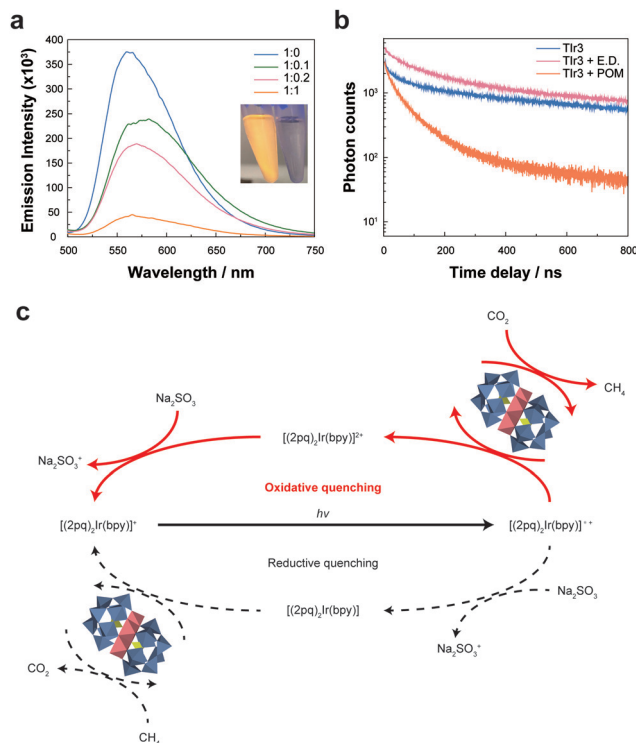
Fig. 3 Photophysical analysis of photocatalytic CO_2RR systems. (a) Static photoluminescence spectra of TlR3 ( 50 \mu\text{M} ) without (blue line) and with ZnPOM at different concentration ratios of TlR3 and ZnPOM. The inset shows a photograph of TlR3 solutions under UV light without (left) and with (right) ZnPOM ( 50 \mu\text{M} ). (b) Time-correlated single-photon counting for lifetime measurements of TlR3 without and with POM or sacrificial electron donor (E.D.) Na_2SO_3 . (c) A suggested mechanistic pathway for the photocatalytic CO_2RR to CH_4 using ZnPOM and TlR3.
