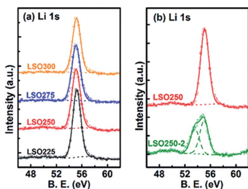
Fig. 12 Deconvolution of Li 1s XPS spectra of lithium silicate thin films deposited (a) at different temperatures and (b) with different Li subcycle numbers. 33
