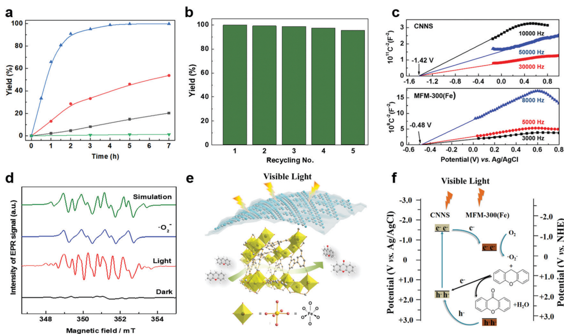
Fig. 2 (a) Formation of xanthone catalysed by MFM-300(Fe) (black), g\text{-C}_3\text{N}_4 (red), CNNS/MFM-300(Fe) composites (blue) and thermal catalysis with CNNS/MFM-300(Fe) composites at 343 K in the dark (green). (b) Catalytic performance over five continuous cycles of oxidation of xanthene. (c) Mott-Schottky plots for CNNS (top) and MFM-300(Fe) (bottom) at different frequencies. (d) EPR spectra spin-trapping with DMPO of CNNS/MFM-300(Fe) under dark conditions (black) and after 10 min of visible light irradiation (red). Signals for \text{O}_2^- (blue) and simulated (green) of the spectrum after irradiation. (e) Schematic diagram for the photocatalytic process. (f) Schematic illustration of charge separation of CNNS and MFM-300(Fe) and charge-transfer between the bands of CNNS/MFM-300(Fe) heterojunctions. The CNNS/MFM-300(Fe) composites shown here contain g\text{-C}_3\text{N}_4 :MOF in a wt:wt ratio of 7:3.
