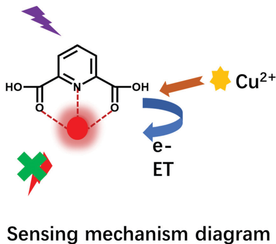
Fig. 7 The sensing mechanism of the fluorescence quenching of the \text{Cu}^{2+} ions.
