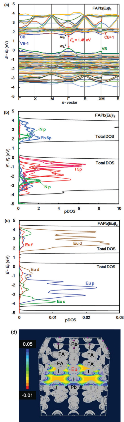
Fig. 1 (a) Band structure, (b) partial density of state, and (c) enlarged view of the 3p, 3d, and 4f orbitals of \text{Eu}^{3+} in the FAPb(Eu 3+ )I 3 perovskite crystal. (d) Contour map of the electron density distribution.
