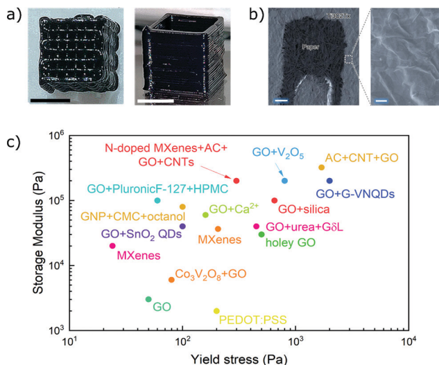
Fig. 10 (a and b) Pictures of structures printed from Ti_3C_2T_x inks (adapted with permission from ref. 73, Copyright 2019 John Wiley and Sons, and from ref. 24, Copyright 2019 Springer Nature); (c) plot comparing the storage modulus and yield stress of DIW inks based on graphene oxide and MXenes (references in Table 1).
