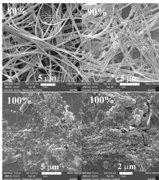
Fig. 4 SEM images of 3 at different water fractions in a \text{CH}_3\text{CN} -water mixture (scale bar = 1 \mu\text{m} ).
