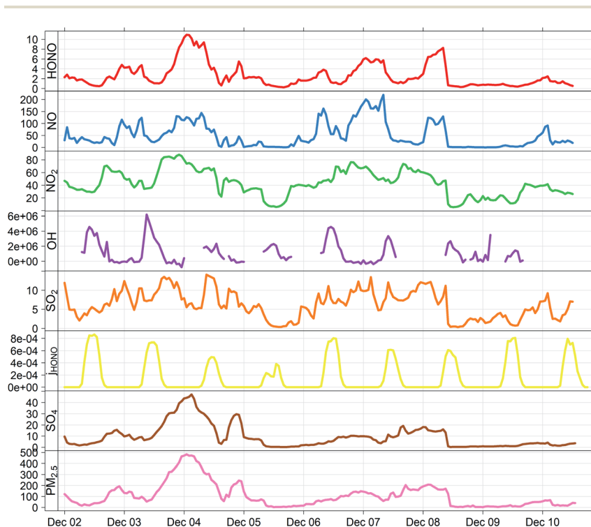
Fig. 1 Measured timeseries for HONO (ppb), NO (ppb), NO_2 (ppb), OH ( \text{molec cm}^{-3} ), SO_2 (ppb), j_{\text{HONO}} ( \text{s}^{-1} ), SO_4 (AMS; \mu\text{g m}^{-3} ) and PM_{2.5} (TEOM FDMS; \mu\text{g m}^{-3} ) at the IAP tower site during the APHH Beijing winter campaign, 2016.
