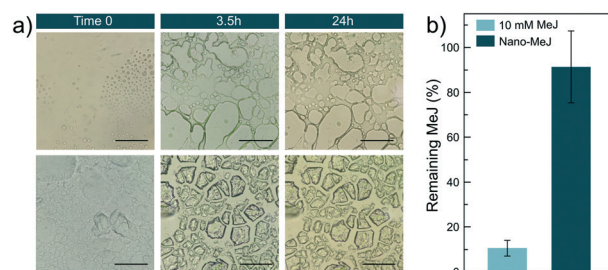
Fig. 6 (a) Optical micrographs of drops containing MeJ (top) and nano-MeJ (bottom) collected at different time intervals at 50 °C. Scale bar = 100 μm. (b) Percentage of remaining MeJ (quantified by UV-vis spectroscopy) after 24 hours at 50 °C for both treatments.
