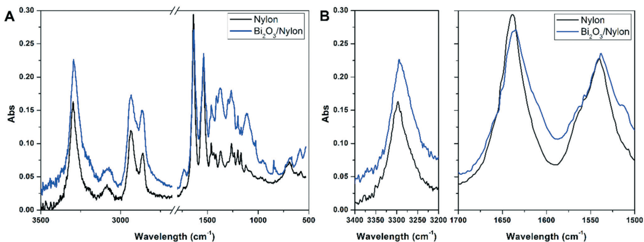
Fig. 4 FT-IR patterns of nylon and \text{Bi}_2\text{O}_3/\text{nylon} membranes: A) whole FT-IR spectrum; B) magnification of the N-H stretching (left) and amide I and amide II (right) regions.
