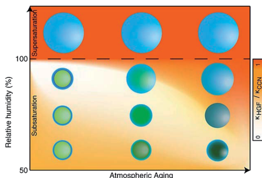
Fig. 34 Schematics of the water uptake processes of SOA particles in the atmosphere. Subsaturated swelling ( K_{HGF} ) can vary dramatically with minor differences in supersaturated droplet activation ( K_{CCN} ); consequently, particles can have very different direct and indirect climate effects. The background color scale indicates the ratio of these parameters under the given subsaturated and supersaturated conditions, whereas the darkness of the green color in particles denotes their atmospheric age. The contrast is the largest when adsorption is the dominant water uptake mechanism even at high RH. This is the case for low O : C SOA particles on the left. With increasing oxidation, i.e. , increasing atmospheric age of the particles, the solubility increases and the dissolution RH decreases, decreasing the discrepancy between the K_{HGF} and K_{CCN} values. Reproduced from ref. 326 under Create Commons License (CC BY-NC-ND 4.0) from the American Geophysical Union, © The Authors, 2015.
