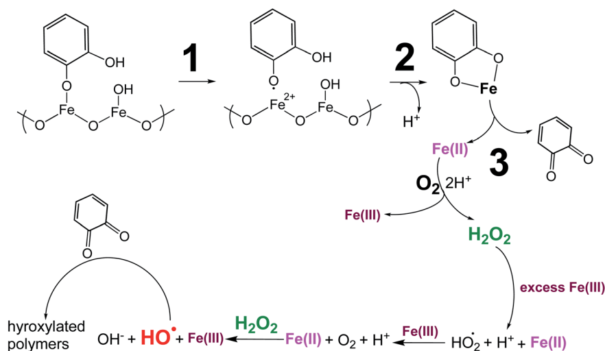
Scheme 5 A three-step mechanism for abiotic oxidative polymerization of catechol on the surface of iron oxide proposed by Colarieti et al. 254 and Larson and Hufnal Jr. 217 The different colors are used to highlight the oxidation state of the iron in the respective step. The larger size of OH and H 2 O 2 is used to highlight the reactive oxygen species generated in the reaction. Reproduced from ref. 206 with permission from the American Chemical Society, © 2020.
