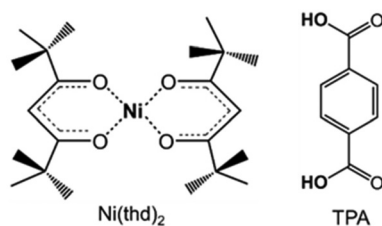
Fig. 1 Molecular structures of the precursors employed in this study.
