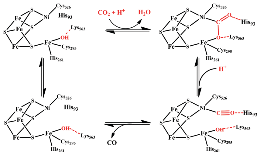
Scheme 4 Proposed mechanistic cycle of \text{CO}_2 reduction to CO by [\text{NiFe}]\text{CODHs} .
