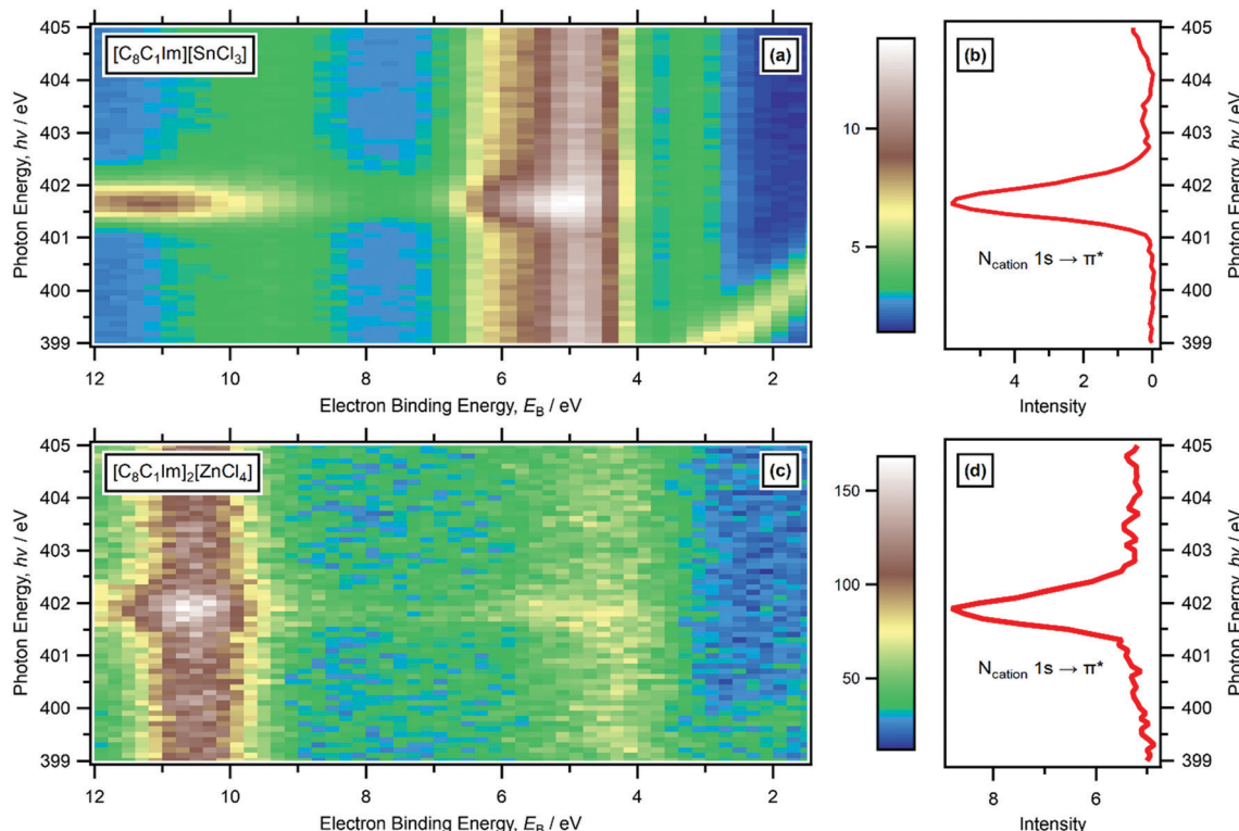
Fig. 3 RXPS N 1s edge data. [C_8C_1Im][SnCl_3] : (a) heat map of h\nu against E_B for the N 1s edge; (b) partial electron yield NEXAFS spectrum for the N 1s edge. [C_8C_1Im]_2[ZnCl_4] : (c) heat map of h\nu against E_B for the N 1s edge; (d) partial electron yield NEXAFS spectrum for the N 1s edge. These RXPS plots represent the raw data, with no subtraction performed. All electron spectra were charge referenced using methods outlined in Section 2.4. The features at 399 eV < h\nu < 401 eV and 0 eV < E_B < 3 eV were due to N 1s photoemission from 2nd order light.
