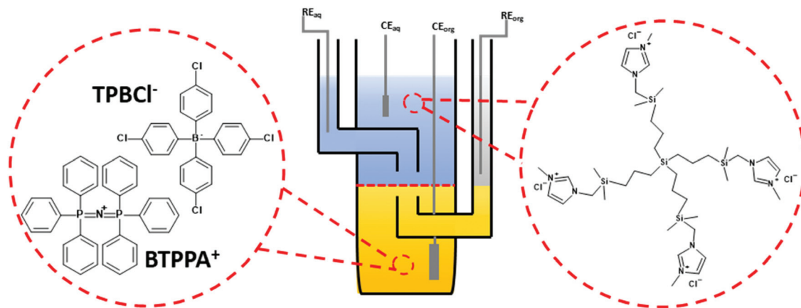
Fig. 1 The electrochemical cell which was used to study the interfacial behavior of imidazolium terminated carbosilane dendrimers. Left: structure of the BTPPA + TPBPCl - being the organic phase (bottom phase) background electrolyte. Right: structure of the G1 dendrimer, which similarly to other members of the family, was always initially dissolved in the aqueous phase. RE – reference electrode, CE – counter electrode, aq – the aqueous phase, and org – the organic phase. The red dashed line in between two Luggin capillaries indicates the position of the ITIES.
