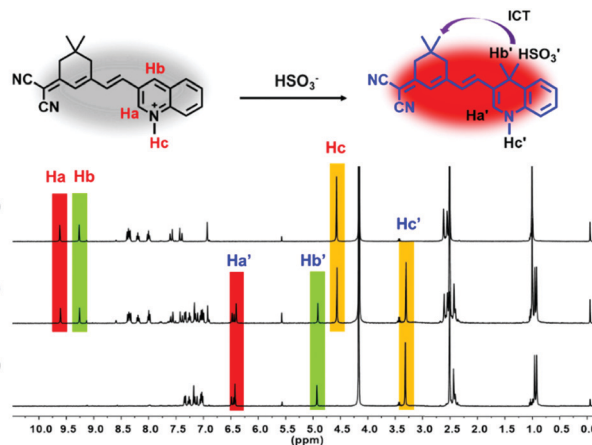
Fig. 4 ^1\text{H} NMR spectra of DCQN with (a) 0 equiv., (b) 9 equiv., and (c) 18 equiv. of \text{HSO}_3^- .
