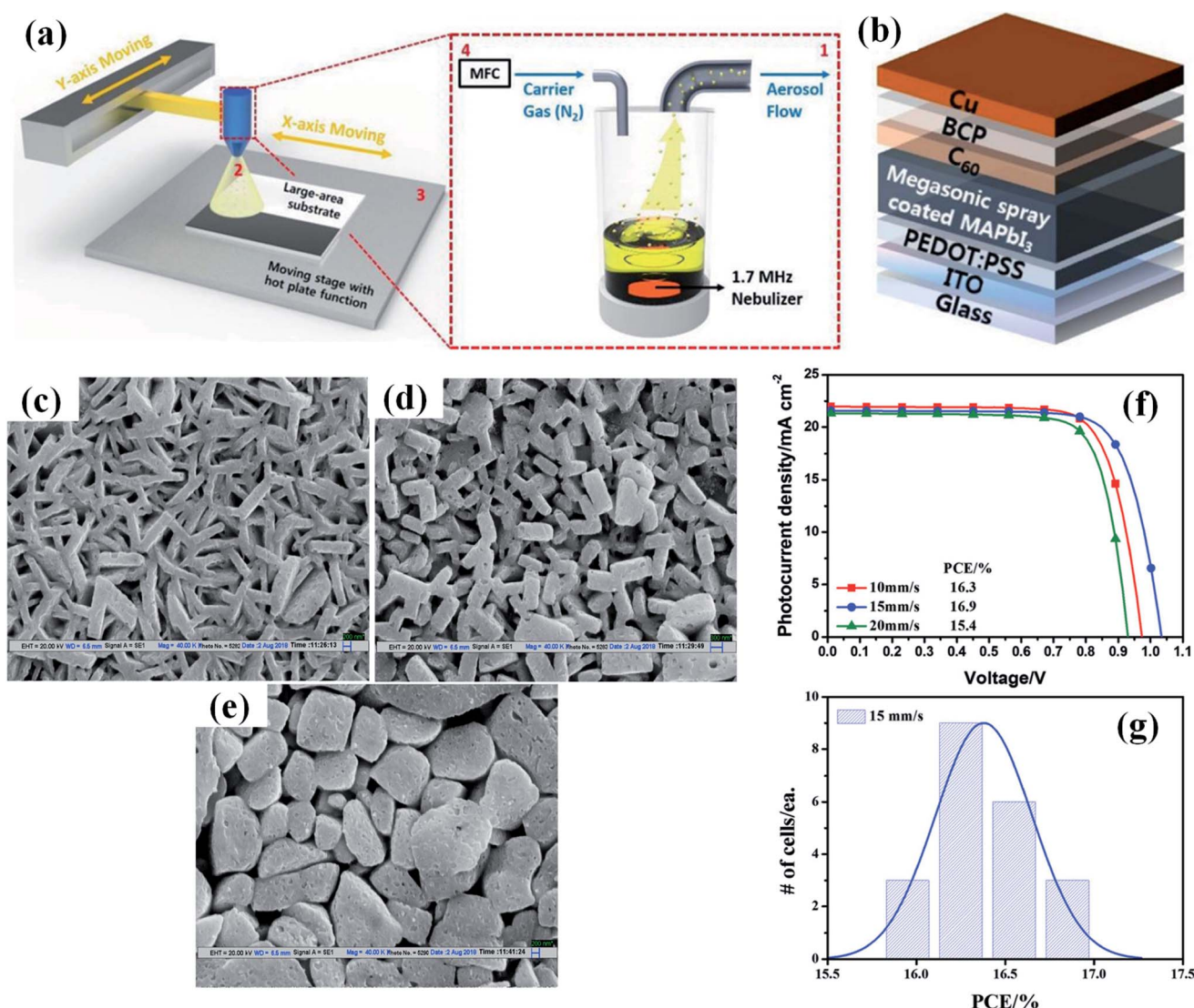
Fig. 27 (a) Schematic illustration of the megasonic spray-coating method. (b) Device configuration of an inverted planar \text{MAPbI}_3 PSC produced by the megasonic spray-coating method. Reproduced by permission ref. 173, Copyright 2018 Wiley-VCH Verlag GmbH & Co. KGaA, Weinheim. SEM image of lead free \text{MA}_3\text{Bi}_2\text{I}_9 perovskite films at different bias during the deposition (c) 0 V (d) 500 V (e) 1000 V. Reproduced by permission ref. 170, Copyright 2019 International Solar Energy Society. (f) Current–voltage characteristics of the best performing devices with three different coating scan speeds. (g) Histogram of photovoltaic performance under 1 sun illumination of 21 samples with a coating scan speed of 15 \text{mm s}^{-1} . Reproduced by permission ref. 173, Copyright 2018 Wiley-VCH Verlag GmbH & Co. KGaA, Weinheim.
