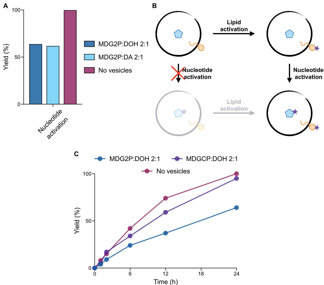
Fig. 4 Evaluation of the compatibility of phospholipid-based vesicles and activation chemistry. (A) Plot reporting the yield (%) of nucleotide ( A3'P ) activation in the absence and presence of vesicles composed of MDG2P after 24 h in DCI buffer, pH 6. (B) Schematic representation of the two potential reaction pathways leading to the activation of both lipids and nucleotides. The preferential pathway describes the selectivity of lipid activation, followed by nucleotide activation. (C) Plot representing the yield (%) of nucleotide ( A3'P ) activation in the presence of phospholipid-based vesicles in DCI buffer, pH 6. The profile of nucleotide activation in the absence of vesicles (dark pink line) is reported for comparison. Plotted data are representative of ^{31}P -NMR experiments.
