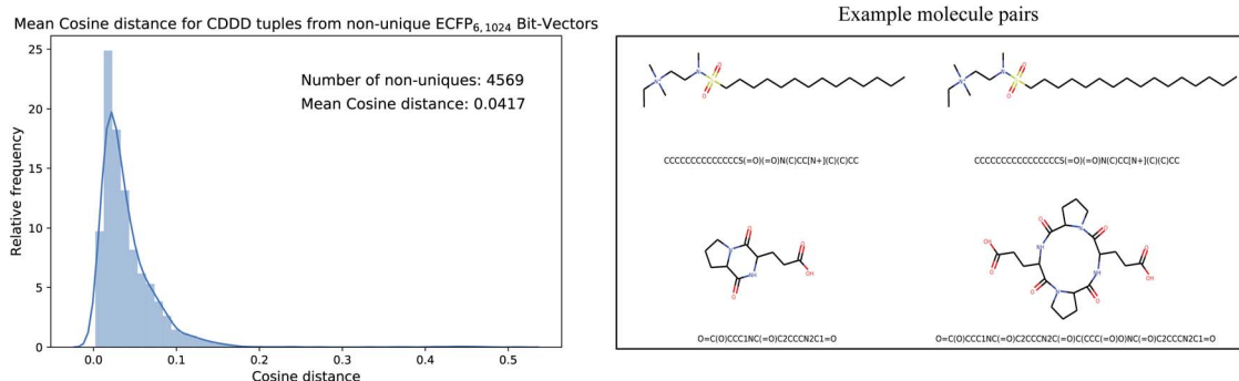
Fig. 4 Mean cosine distance between cddd-representations that belong to the same set of SMILES that map to the same ECFP representation. On average, the cosine distance is small with 0.0417.
