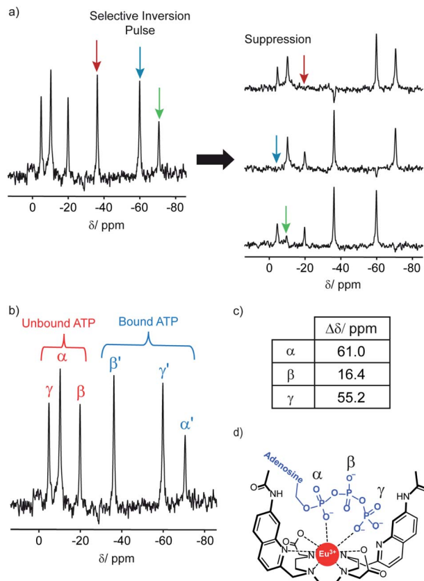
Fig. 4 ^{31}\text{P} NMR (202.21 MHz) of ATP (6.57 mM) with [\text{Eu.1}]^+ (6.57 mM) in 1 : 1 \text{D}_2\text{O} : MeOD, pH 7.0, indicating bidentate binding of ATP to the europium(III) ion. (a) ^{31}\text{P} NMR selective inversion experiment, wherein selective inversion of one of the bound ATP ^{31}\text{P} signals leads to suppression of the corresponding unbound ^{31}\text{P} signal, due to rapid exchange on the NMR timescale. (b) ^{31}\text{P} NMR of ATP + [\text{Eu.1}]^+ , showing ^{31}\text{P} signals for both bound and unbound ATP. (c) Change in chemical shift for the \alpha , \beta and \gamma -phosphates between the bound and unbound ^{31}\text{P} NMR signals. (d) Proposed bidentate binding mode of ATP to [\text{Eu.1}]^+ , via the \alpha and \gamma -phosphate groups.
