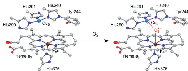
Scheme 1 Illustration of the O_2 binding and activation at the dinuclear heme a_3 and Cu_B site of CcO.
