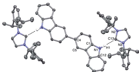
Fig. 3 ORTEP diagram (ellipsoids drawn at 50% probability) of BC...2IPr . Non-hydrogen bonding hydrogens and co-crystallized \text{THF} are omitted for clarity. Average select bond lengths (Å) and angles ( ^\circ ): \text{H1}\cdots\text{C13} , 2.10; \text{N1}\cdots\text{C13} , 2.96; \text{N2}-\text{C13}-\text{N3} , 102.2^\circ ; \text{N2}-\text{N3}-\text{C12}-\text{C1} , 13.5^\circ .
