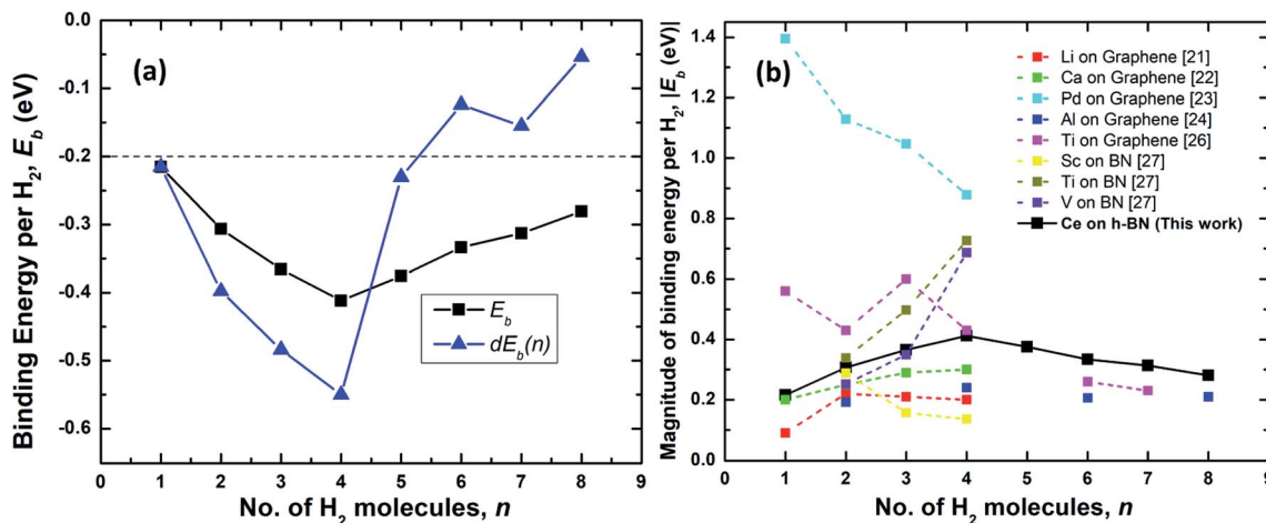
Fig. 4 (a) Binding energy per hydrogen molecule on Ce decorated h-BN, E_b^n (black squares) and energy required to add n th hydrogen molecule, dE_b^n (blue triangles) over Ce decorated h-BN. The dashed line represents the upper limit of the US DOE target for ambient hydrogen storage; the lower limit being at -0.7 eV. 53 (b) Comparison of the absolute value of average binding energy, |E_b| as number of hydrogen molecules is increased for other metals decorated on 2D materials – graphene and borazine as reported in literature.
