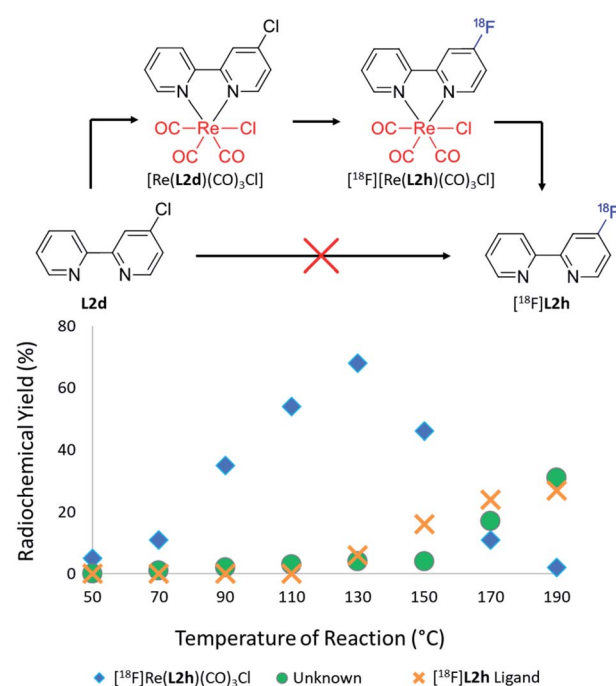
Fig. 4 RCYs of [\text{Re}(\text{L2h})(\text{CO})_3\text{Cl}] (blue diamonds), [\text{Re}(\text{L2d})(\text{CO})_3\text{Cl}] (orange crosses) and an unknown by-product (green circles) plotted as a function of the reaction temperature for the [\text{Re}(\text{CO})_3(\text{L2d})\text{Cl}] complex. [\text{Re}(\text{L2h})\text{L2h}] was unable to be synthesised from \text{L2d} unless mediated by rhenium(i) complexation as per the above scheme.
