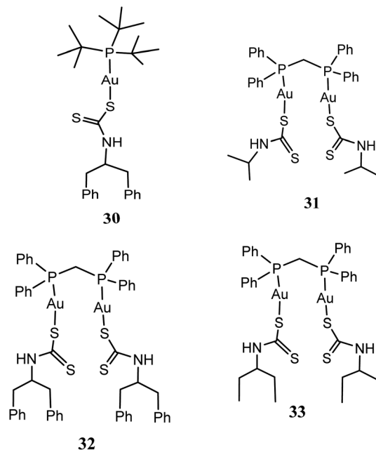
Fig. 6 Chemical structures of phosphine gold(i) dithiocarbamate complexes 30–33.
