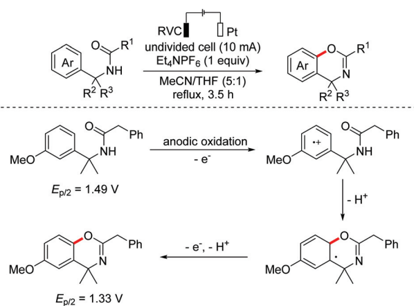
Scheme 74
