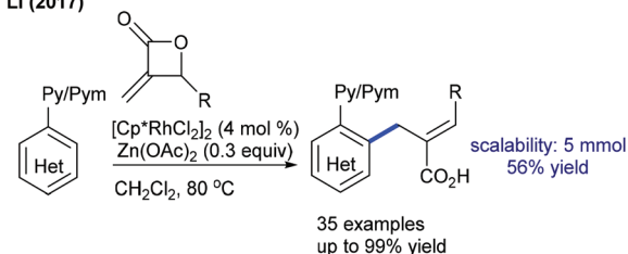
Scheme 137 Redox-neutral coupling of methyleneoxetanones with arenes.
