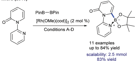
Scheme 103 C6-Borylation of pyridones.
